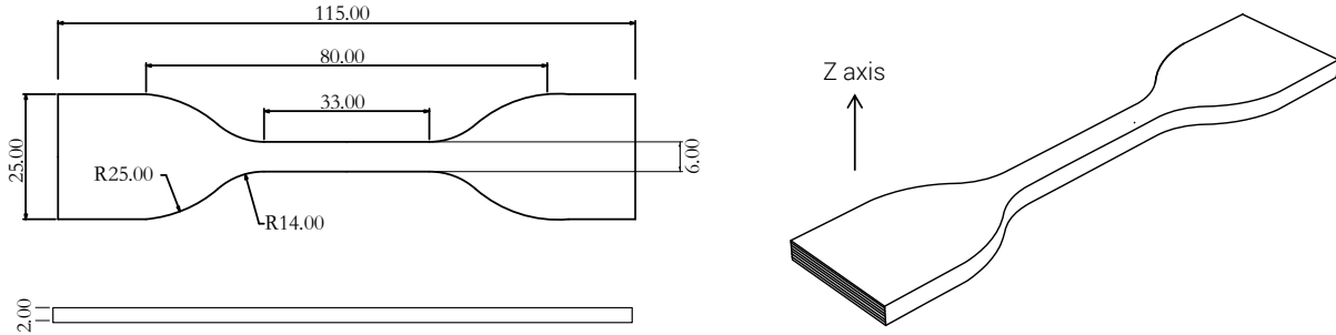
Tensile testing specimen; ASTM D638 (ISO 527, GB/T 1040)
