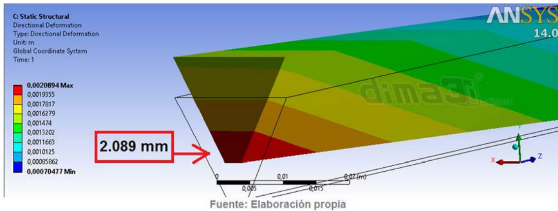
Figure 10. Deformation caused by internal tensions printing with regular lacs at 75°C (167°F)
